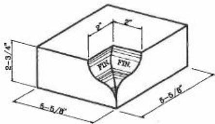
Watertable Internal Corner
