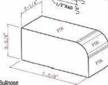
Rowlock Bullnose
