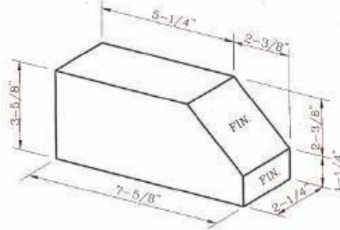
Rowlock Sloped Sill
