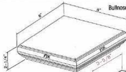
Header Bullnose
