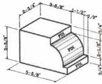
Watertable Rowlock
