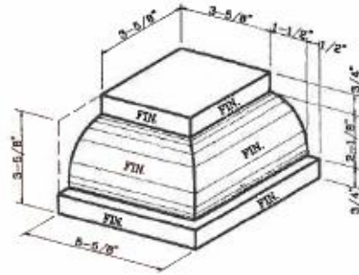
Watertable Rowlock External Corner
