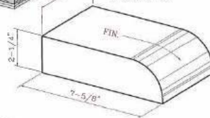
Header Bullnose
