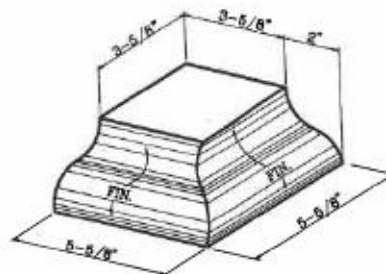
Watertable External Corner
