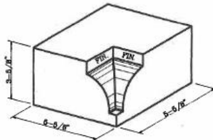
Watertable Rowlock Internal Corner
