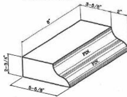
Watertable Stretcher
