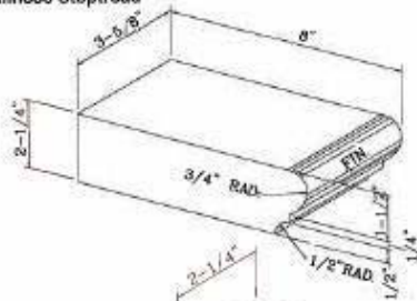
Bullnose Steptread
