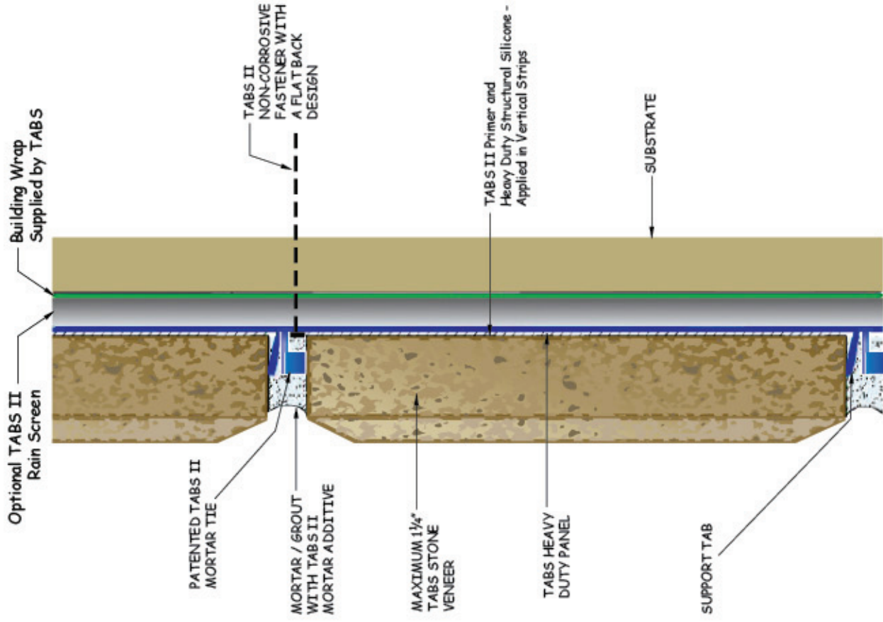
TYPICAL WALL DETAIL With Optional Rain Screen
